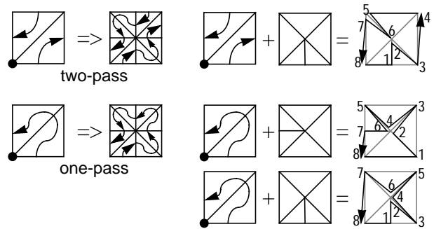
FIGURE 7. Triangle strip decomposition
