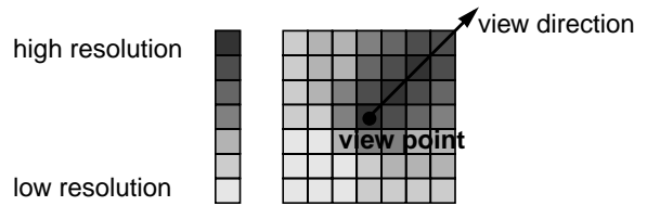
FIGURE 9. LOD distribution
