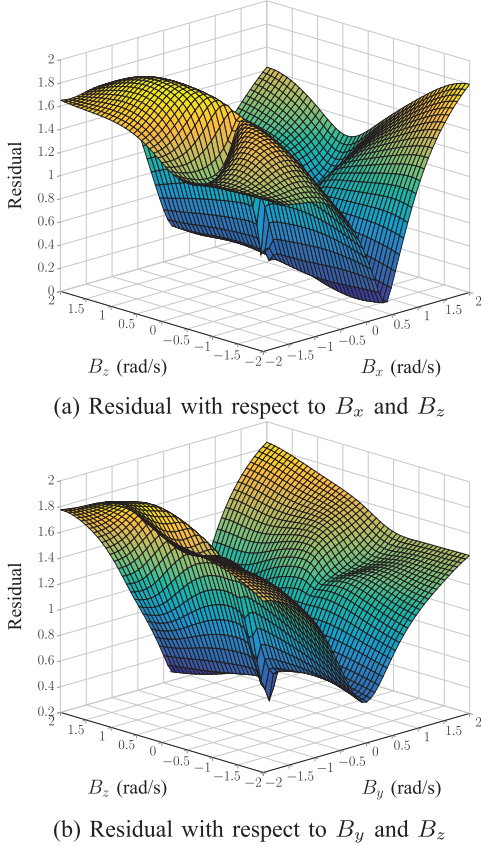
Fig. 7. Cost function (residual) with respect to the gyroscope bias for a small amount of available measurements (integration of 1 second while observing 7 features).
