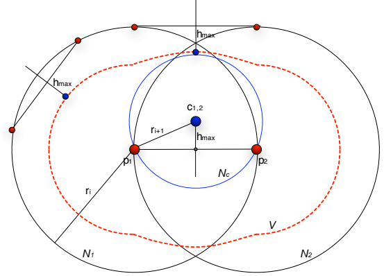
Figure 7: A point created by two parent points outside U are always outside the red region V . As V fully encloses the child's neighborhood N_c of the next refinement step (blue) all candidate neighbor points are known and neighborhoods can be updated correctly.
