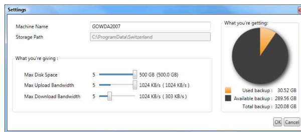
Fig. 1. Screenshot of the Current User Interface: The Settings Window.
