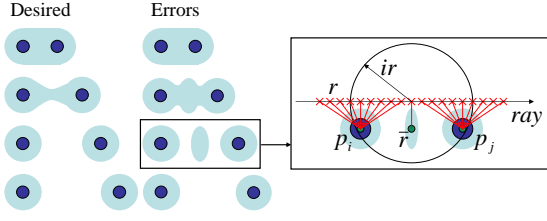
Figure 6: Surface reconstruction errors in the method presented by [ZB05] before postprocessing: when particles are separated by distances comparable to the influence radius, the center of mass may move very quickly leading to surface artifacts.
