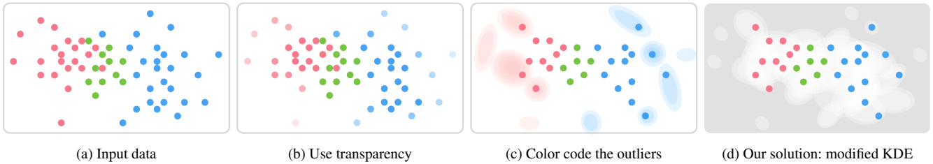
Figure 4: The alternative visual designs of outlier preservation methods.
