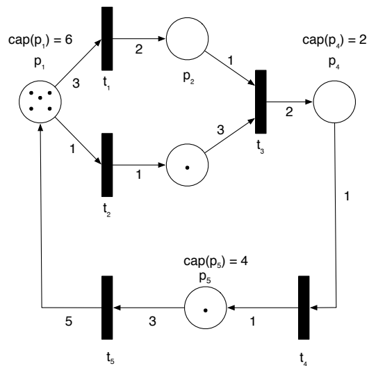
Figure 2: Petri net to be translated in Promela
