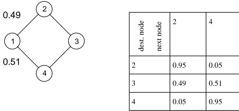
Figure 1: A simple network configuration and the corresponding pheromone table for node 1. Ants traveling from node 1 to node 3 have a 0.49 probability to choose node 2 and a 0.51 probability to choose node 4 as their next node.
